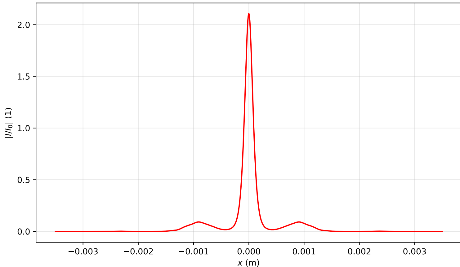
Intensity profile I(x, y = 0, z = 2.149)/I_0 , P_{in}=8.0P_{cr} , artificial time
